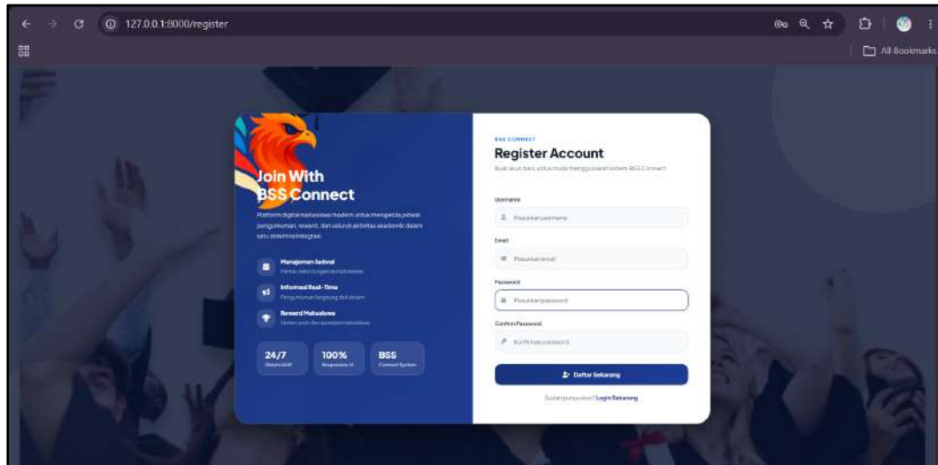
Gambar 4. 3 Halaman Register
