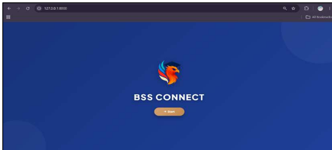
Gambar 4. 1 Landing page
