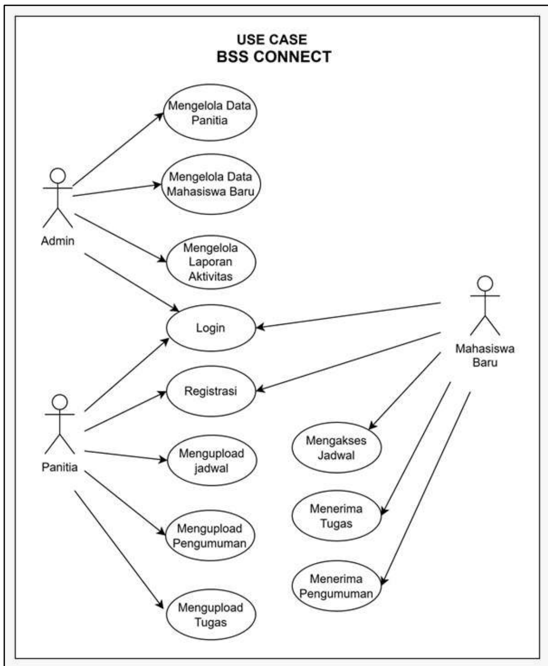
Gambar 3. 1 Use Case
