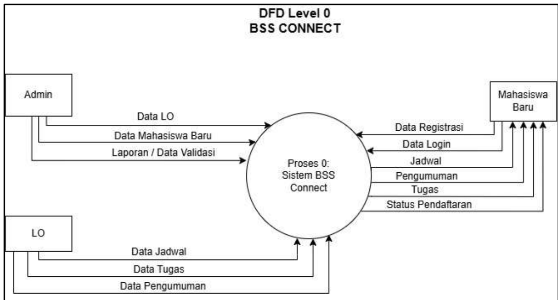
Gambar 3. 3 DFD Level 0
